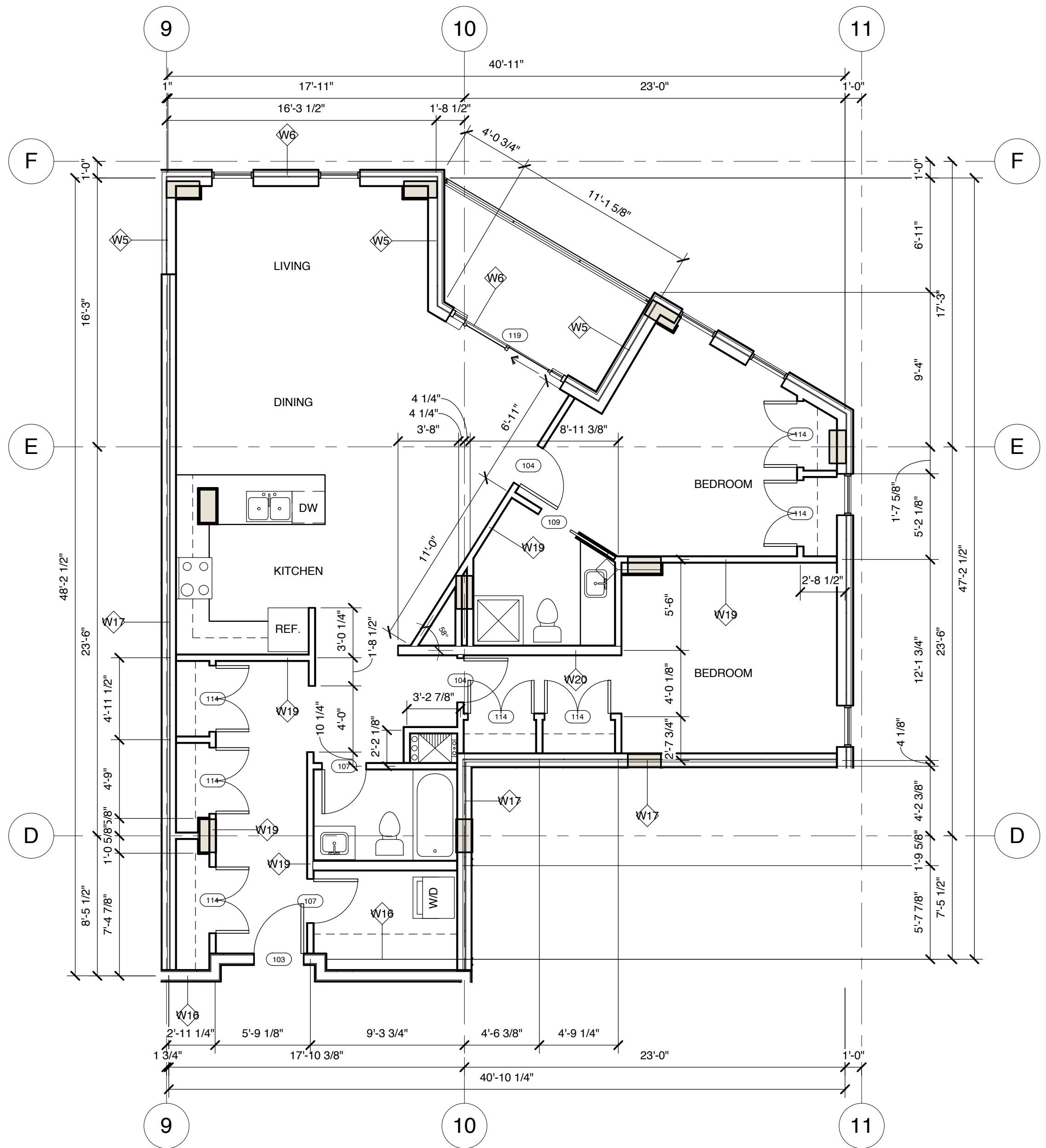
1 Suite Layout C 208-508 3/16" = 1'-0" AREA - 1308 SQ.FT.
