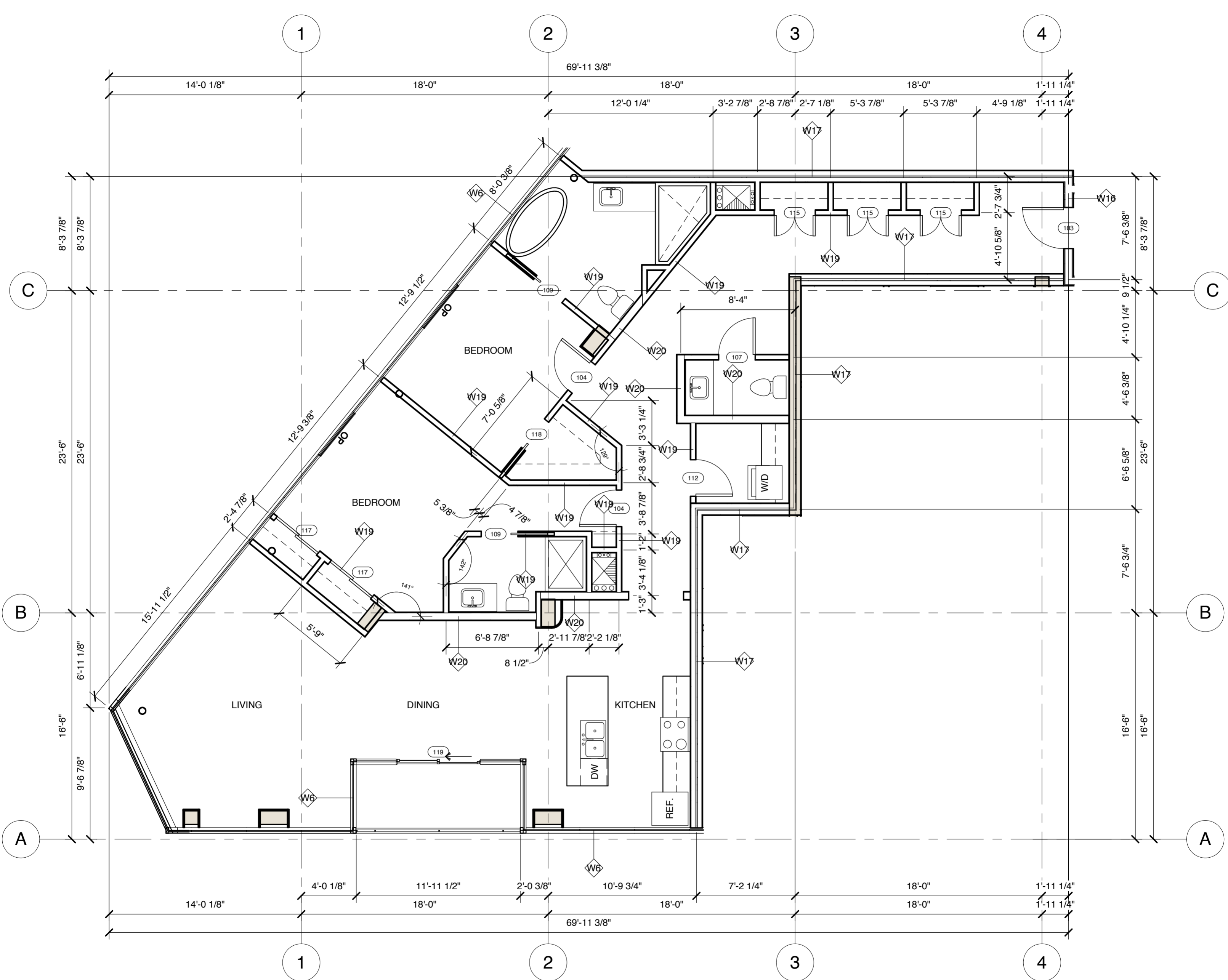
2 Suite Layout D 203-503 3/16" = 1'-0" AREA - 1583 SQ.FT.
