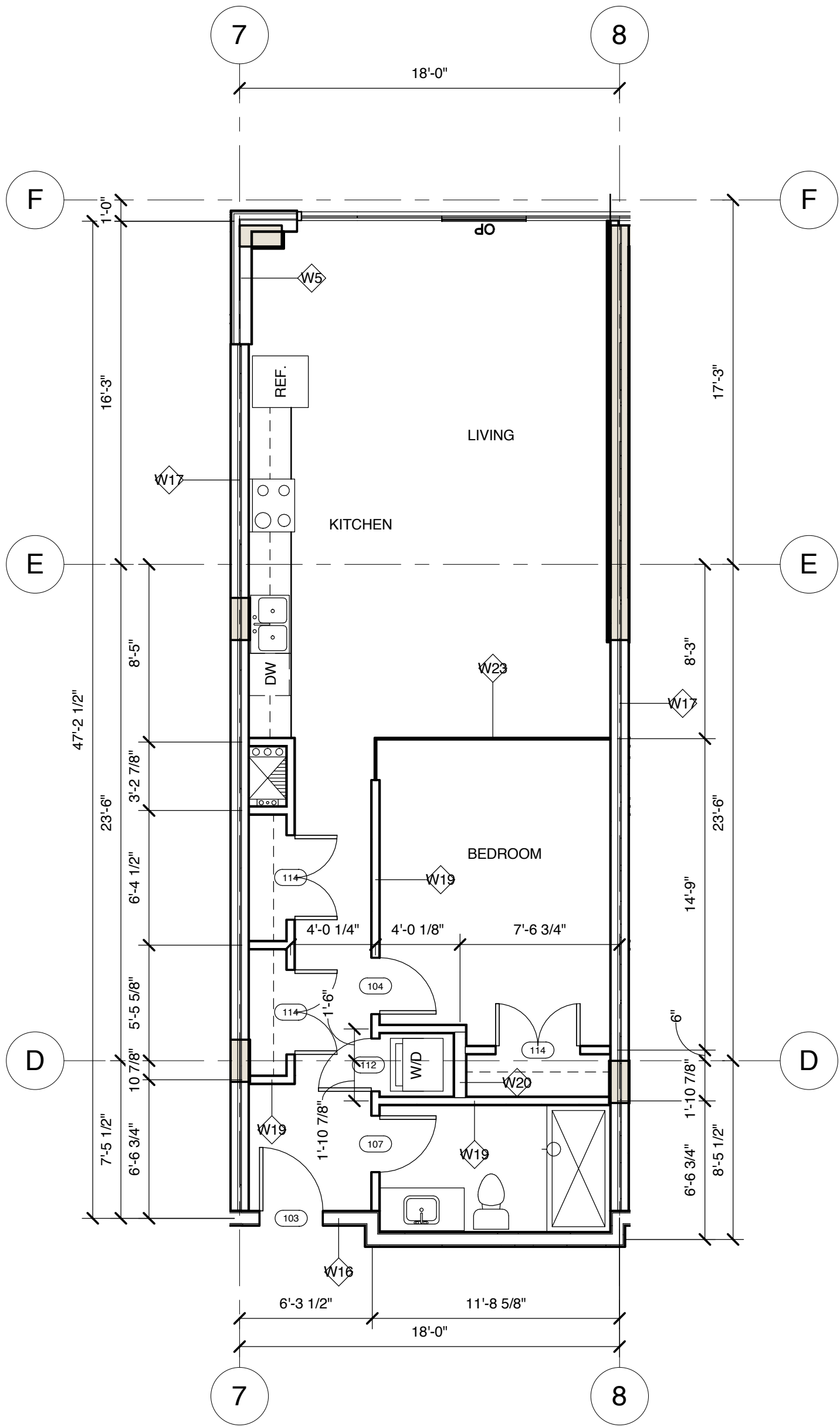
3 Suite Layout G3 3/16" = 1'-0"
