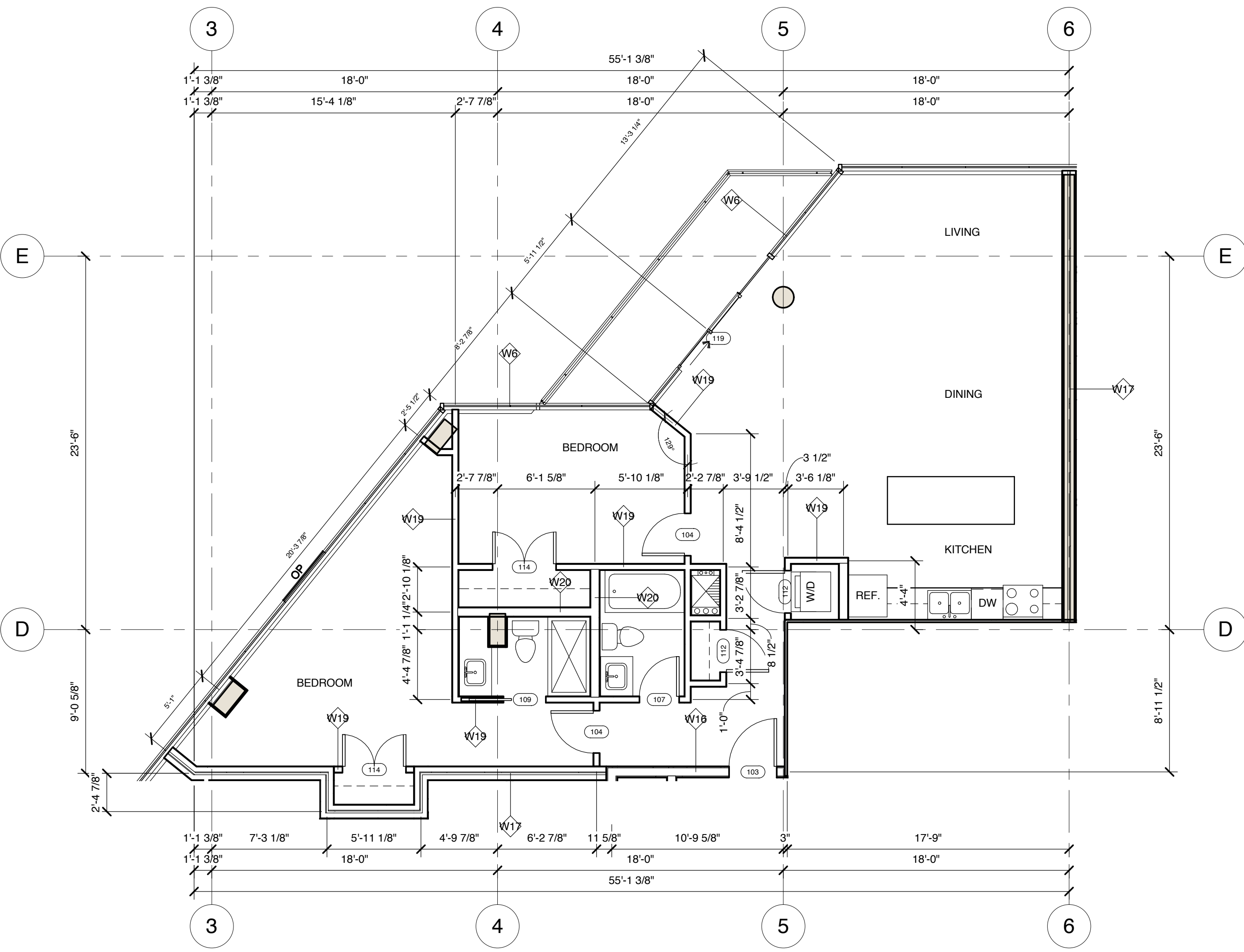
1 Suite Layout K 603-703 3/16" = 1'-0" AREA - 1225 SQ.FT.
